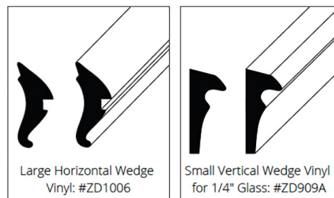
Glazing Vinyl
