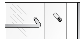
Through-the-glass Towel Bar & Pull with optional concave caps (included)
